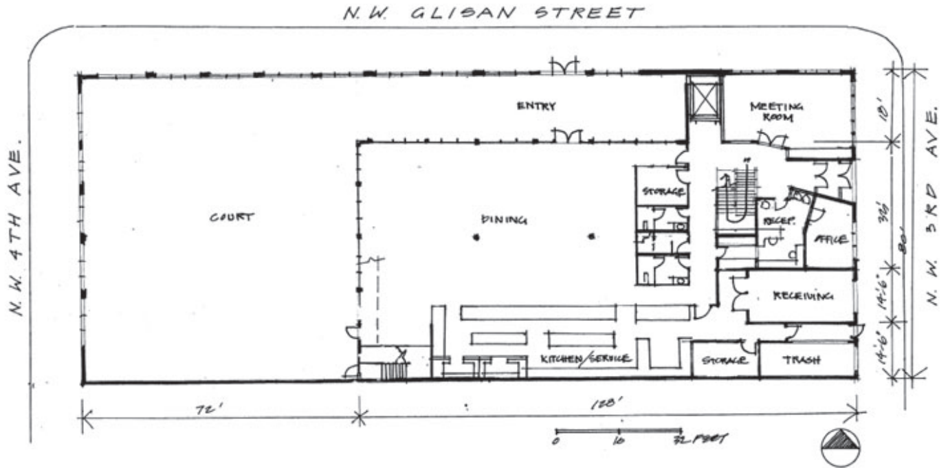
FIRST FLOOR PLAN BLANCHET HOUSE GROUP MACKENZIE MAY 24, 2006 2050294.00
